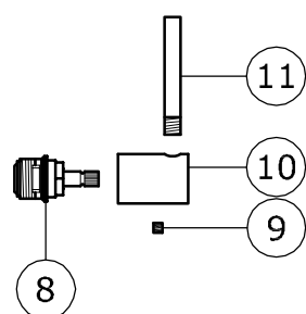
CENTRAL LEVER
