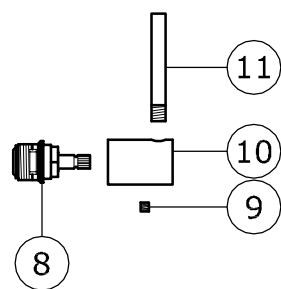
CENTRAL LEVER
