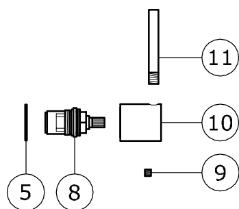
CENTRAL LEVER
